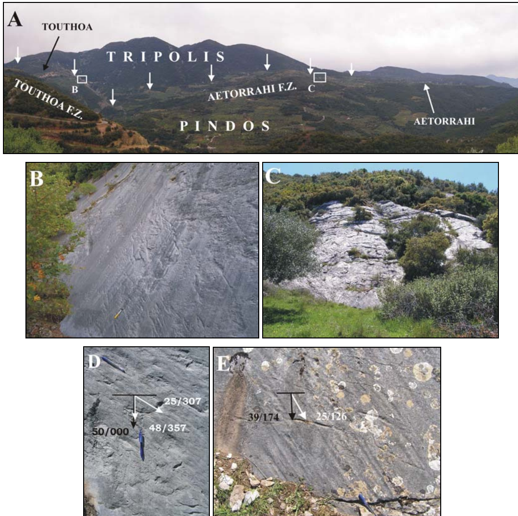
Figure 5: - (A) Panoramic view of Toythoa (TFZ) and Aetorrahi (AFZ) fault zones from northwest. (B) Fault surface of TFZ trending E-W with (D) two sets set of striations. (C) Curved low angle fault surface of AFZ with (E) a set of striations.
