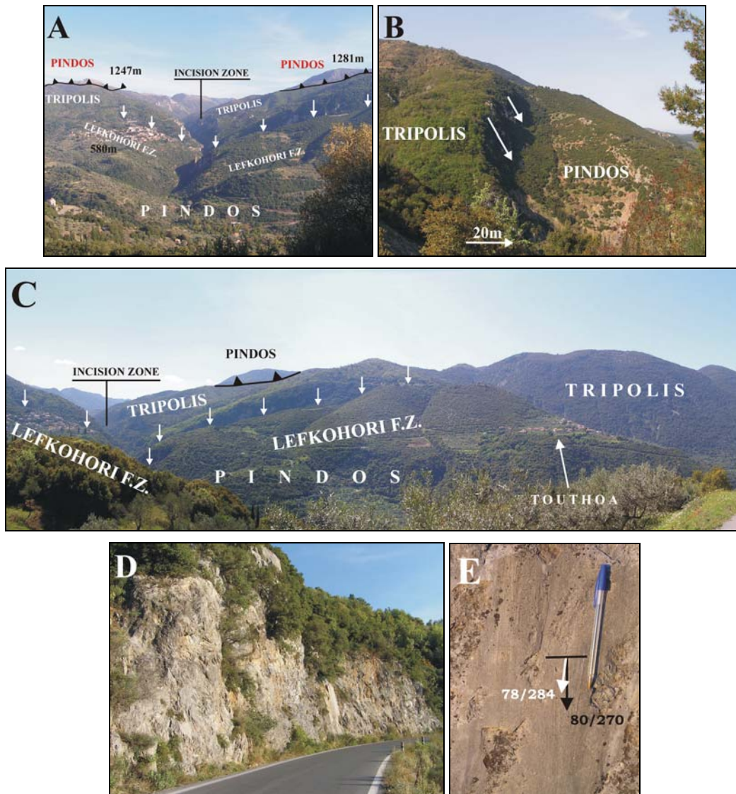
Figure 4: (A) Partial view of LFZ with incision in the impressive canyon of Touthoa River. The remains of Pindos nappe in Lagadia (left) and Servou (right) indicate a vertical displacement at least 700m for LFZ. (B) LFZ forms a large escarpment in the morphology. (C) Panoramic view of LFZ from northwest. (D) A NW-SE striking fault that cut carbonates of the Tripolis unit and (E) fault surface with dip slip striations.
