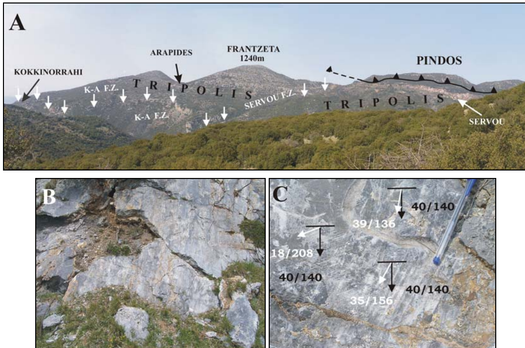
Figure 7: - (A) Panoramic view of Servou (SFZ) and Kokkinorrahi-Arapides (K-AFZ) fault zones with the remains of Pindos nappe in Servou wider area (view from the south). (B) Fault surface of SFZ presenting three sets of striations plunging 35^{\circ}/156^{\circ} , 39^{\circ}/136^{\circ} and 18^{\circ}/208^{\circ} from the older to the younger respectively (C).
