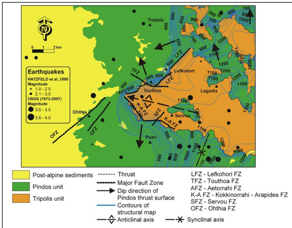
Figure 8: - Structural contour map of the contact between the formations of Pindos and Tripolis geotectonic units and the plot of earthquake epicenters (USGS) in the study area.
