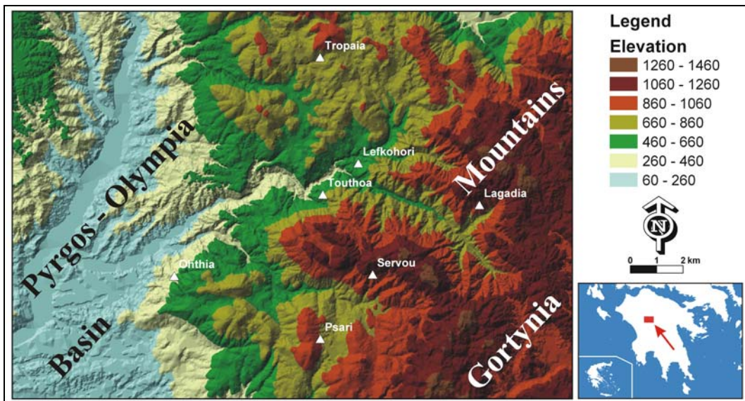
Figure 1: - Gortynia Mts and Pyrgos-Olympia basin as well as the relief of the study area are shown.
