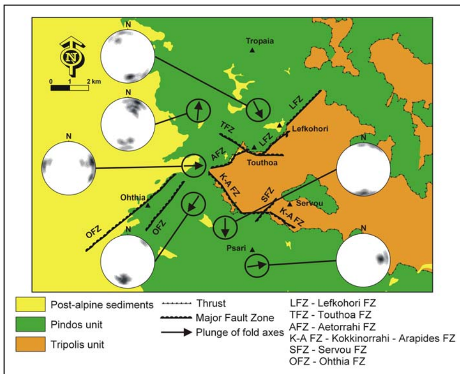
Figure 3: - Structural map showing the tectonic window of Tripolis unit and the main fault zones of the study area as well as the statistical analysis of the fold axes (lower hemisphere, equal area projection) occurring in the Pindos unit formations (see text).
