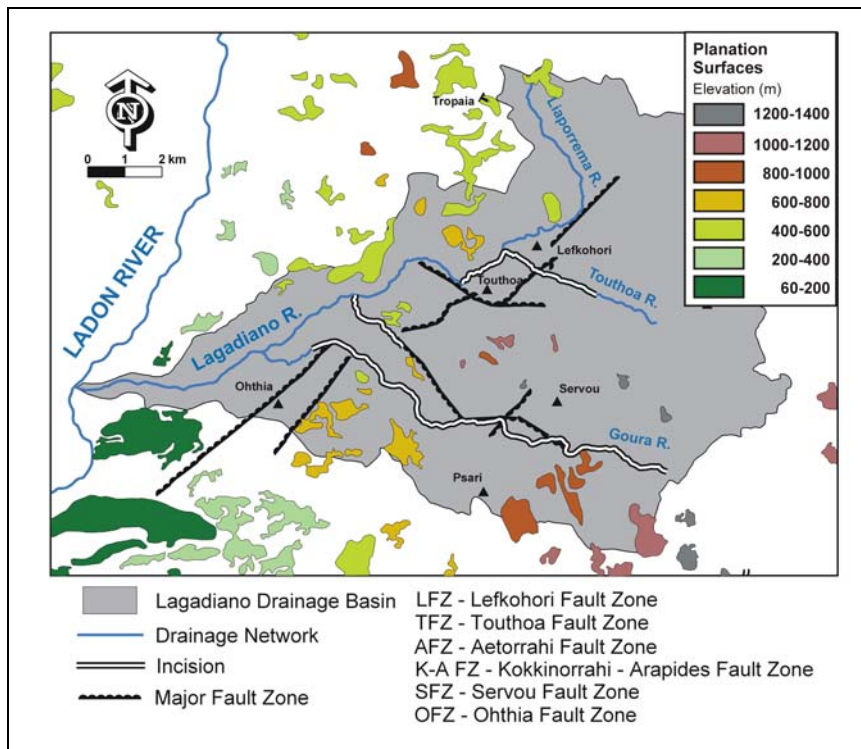
Figure 2: - Map showing the main geomorphic features (planation surfaces, incision zones, and the main tributaries of the drainage network) as well as the major fault zones of the study area.
