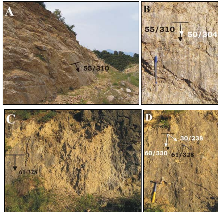
Figure 6: - (A) A NE-SW fault surface of the Ohthia (OFZ) fault zone cutting the limestones of Pindos unit. (B) Tectonic breccia and dip slip striations on it observed on the previous fault surface. (C) A NE-SW fault surface of the same fault zone being the contact between the Pindos limestones and the pleistocene age Erymanthos formation. This surface belongs to the western segment of the OFZ and has (D) two sets of striations.
